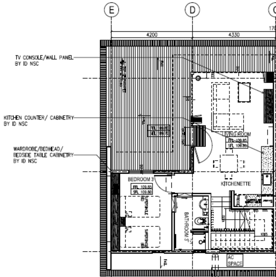
VILLA A/B 1ST STOREY PLAN
